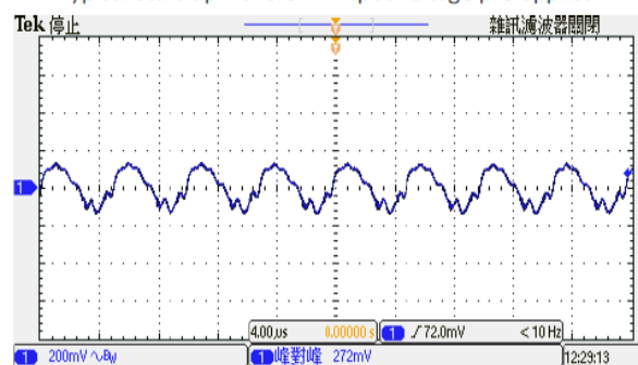
Figure 8 : Output Voltage Ripple & Noise at full load. ( V_{in} : Typical, With Output Capacitor to add 1\mu F MLCC)
